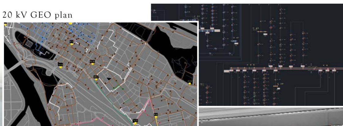
20 kV network diagram
